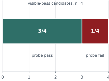
Fig. 6. Quantified certificate evidence for the Matplotlib all-NaN bar-plot case. The public probe splits four visible-passing candidates into three probe-pass and one probe-fail candidates; the record is retained before freeze and receives its false-acceptance label only after held-out calibration.
