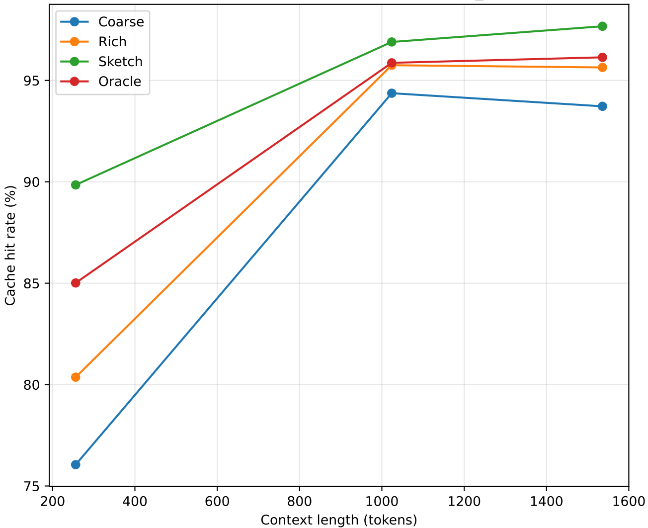
Cache hit rate vs context length (Tier B, tool_delay=0)
