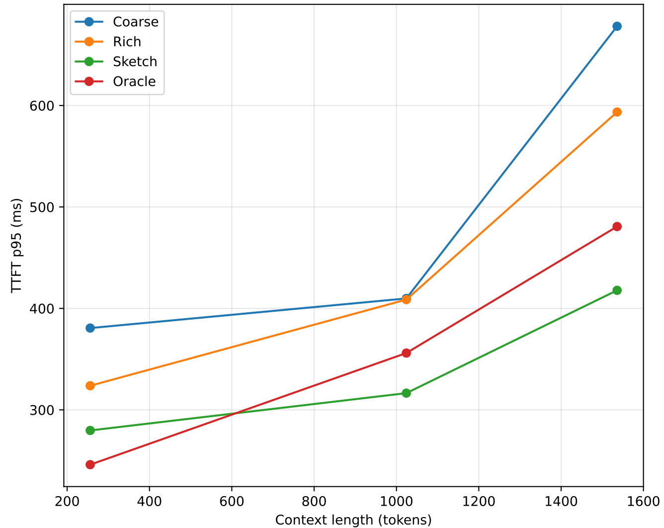
TTFT p95 vs context length
