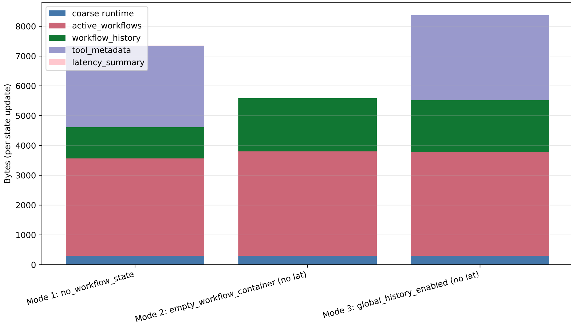
Rich State Size Breakdown by Mode (Tier D, chatbot cells)
