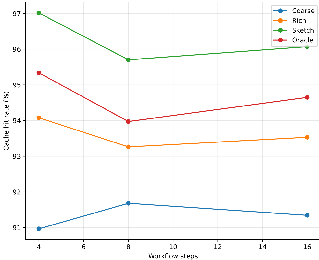
Cache hit rate vs workflow length (Tier C)
