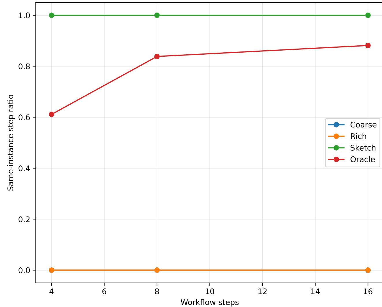
Affinity (same-instance step ratio) vs workflow length
