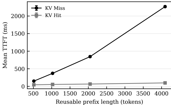
(a) TTFT with and without KV reuse
