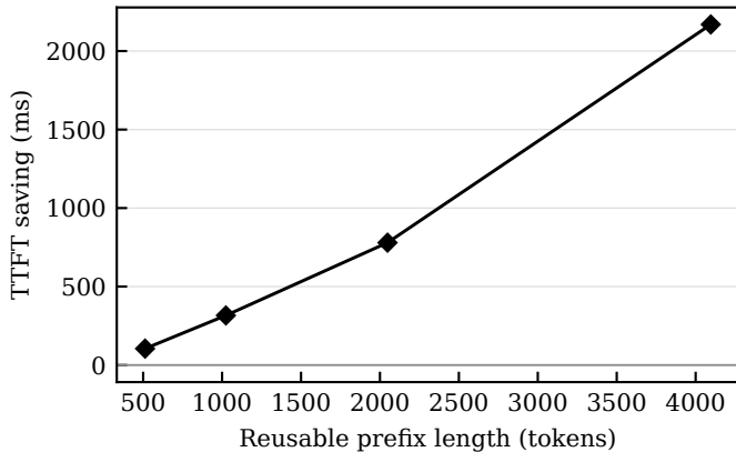
(b) Benefit of KV reuse
