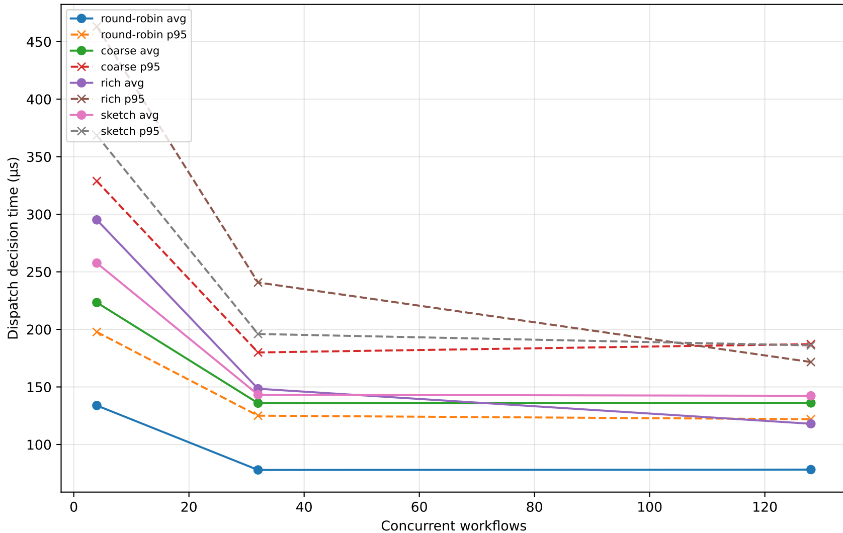
N=256 Dispatch Decision Time vs Concurrency (4 policies × 3 reps × 3 concurrency)
