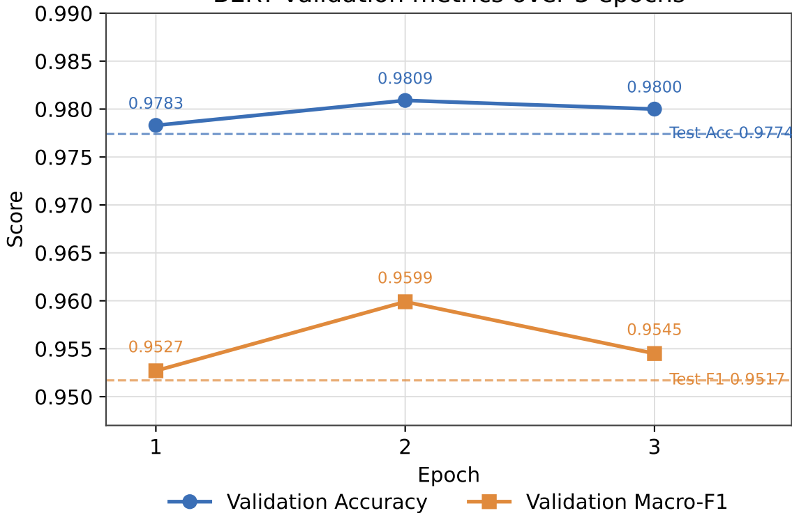
BERT validation metrics over 3 epochs
