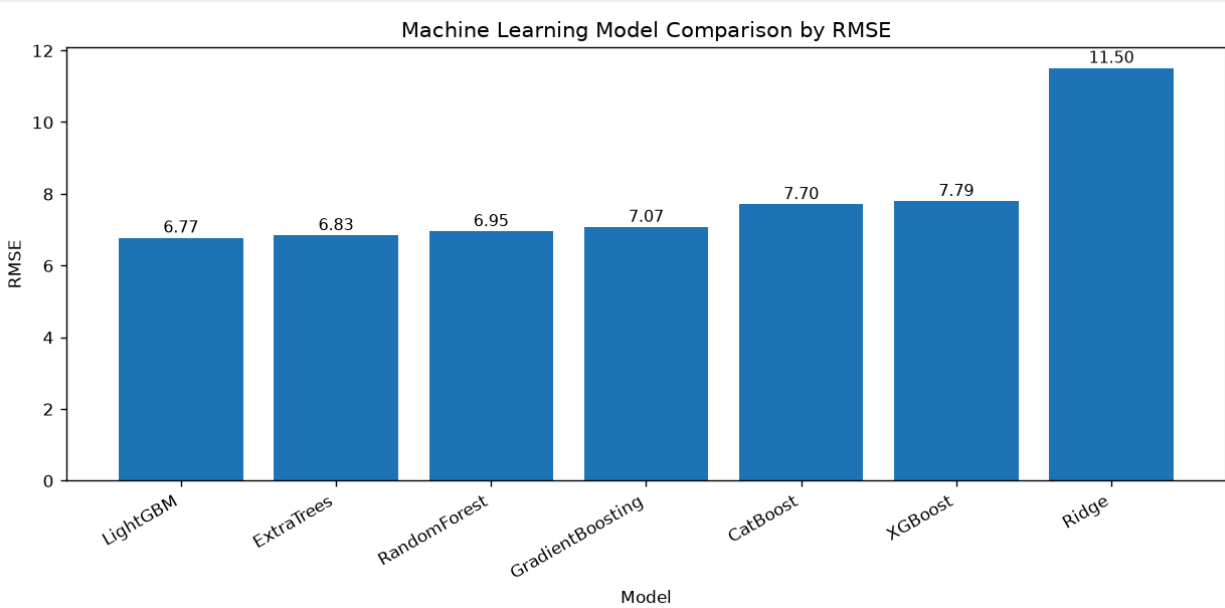
Figure 10. Comparison of conventional model RMSE values.
