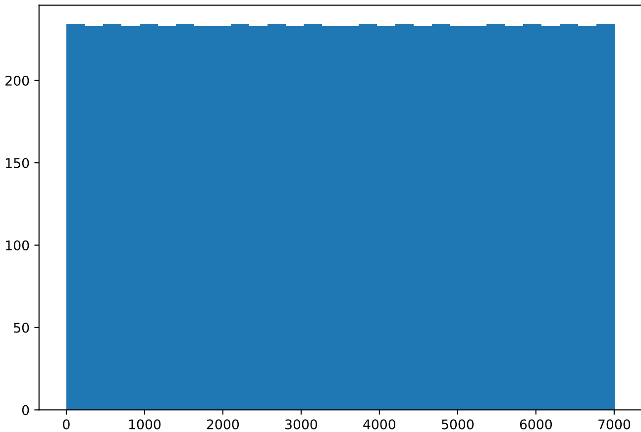
TOPSIS Distribution
