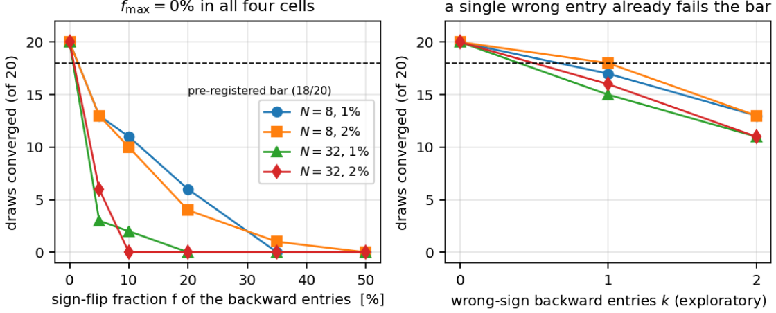
Figure 5: The sign requirement is a hard threshold, not a rate. Left: draws converging to within 2\times the exact-adjoint anchor, against the fraction f of backward entries whose sign is flipped; the flip sets are nested, so the curve is monotone in the flipped set. Right: an exploratory refinement with exactly one and exactly two flipped entries (of 32 at N=8 , of 128 at N=32 ). A single wrong entry already drops convergence below the pre-registered bar in 3 of 4 cells.
