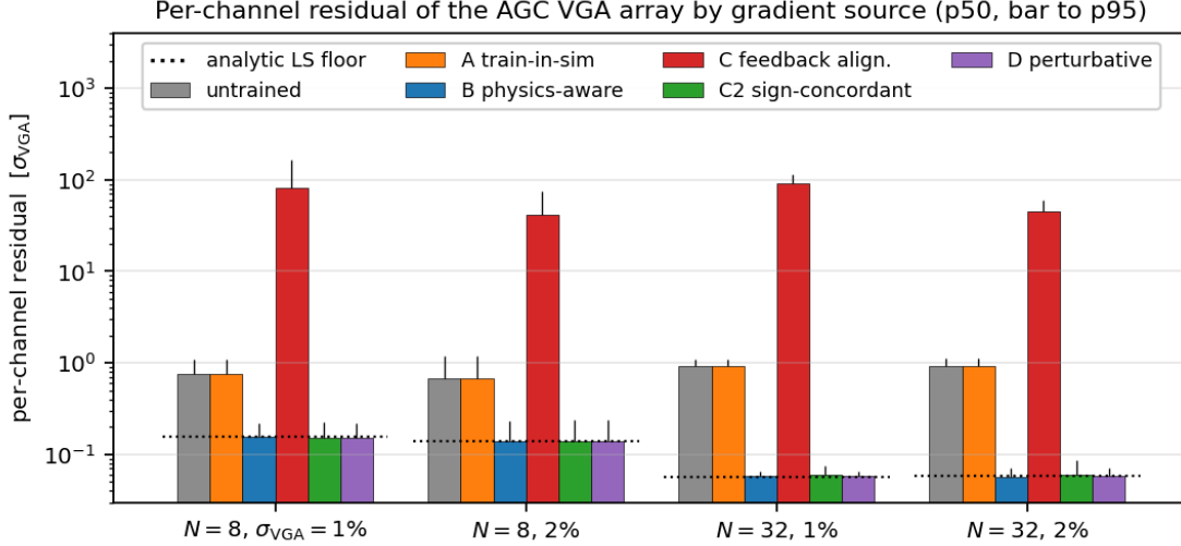
Figure 4: Per-channel residual of the AGC VGA array by gradient source, in units of \sigma_{\text{VGA}} , over 20 Monte-Carlo mismatch draws per cell (bars: median; whiskers to p95; dotted line: the analytic least-squares floor of the training set). Train-in-simulation is bit-for-bit identical to untrained— \gamma converges to 1. Physics-aware, sign-concordant and perturbative gradients all land on the analytic floor. A fully random backward path diverges in every draw of every cell.
