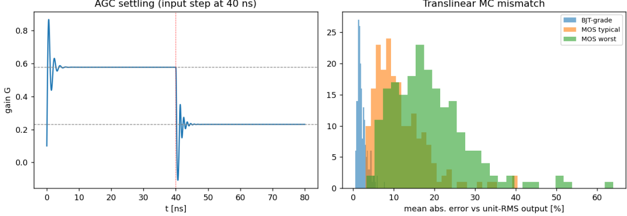
Figure 2: Circuit-level validation. Left: AGC gain transient (ngspice, real 1 pF integration capacitor). The loop settles to the exact RMSNorm gain in 4.4 ns from cold start and re-settles in 5.3 ns after a 2.5\times input step at t = 40 ns (dashed lines: exact targets). Right: Monte-Carlo mismatch distributions for the open-loop translinear pipeline at three technology corners; in the feedback implementation, the corresponding detector-side mismatch shifts only the common-mode gain and produces no per-channel distortion by construction (quantified in Table 10).
