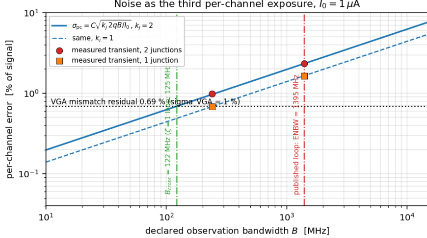
Figure 3: Noise as the third per-channel exposure of the AGC array, at I_0 = 1 \mu\text{A} . Lines: Eq. (3) with C = 0.780 for a one- and a two-junction channel path. Markers: transient measurements on one bench under two bandwidth conventions. Dotted line: the 0.69% VGA mismatch residual of Table 10. Noise equals mismatch at B = 122 \text{ MHz} , which coincides to 2% with the noise bandwidth the published loop has when it is critically damped; at the loop’s actual ENBW of 1395 MHz noise is 3.3\times mismatch.
