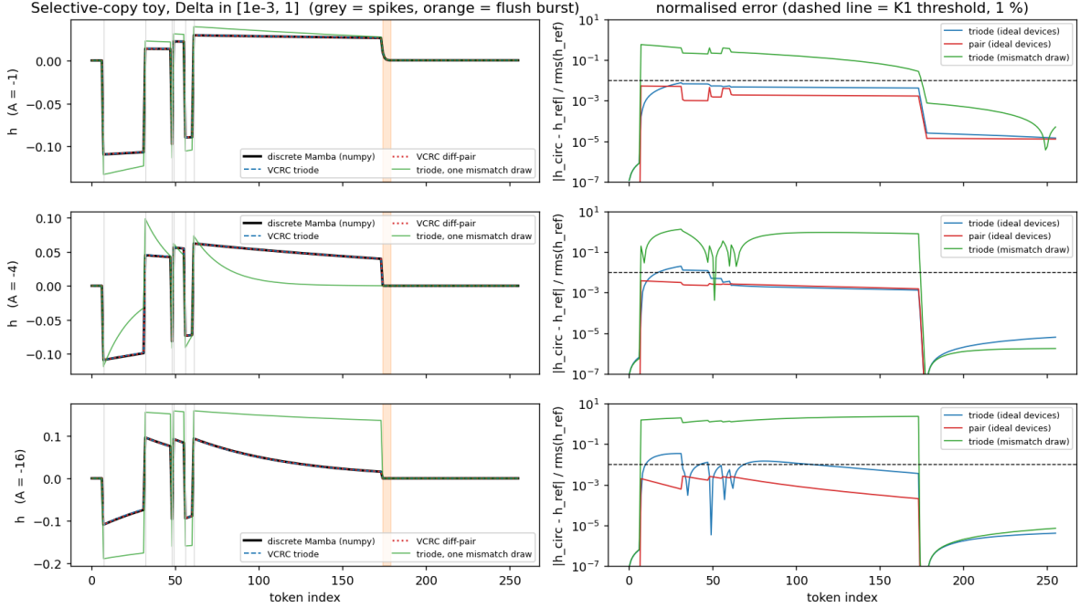
Figure 6: Selective-copy trajectory of the variable- \tau RC realization, \Delta \in [10^{-3}, 1] , three channels ( A = -1, -4, -16 ). Left: state against the discrete selective-scan reference, for both circuit variants and one mismatched triode draw. Right: normalized per-token error on a log axis, with the 1% criterion marked. Selectivity survives mismatch even where precision does not.
