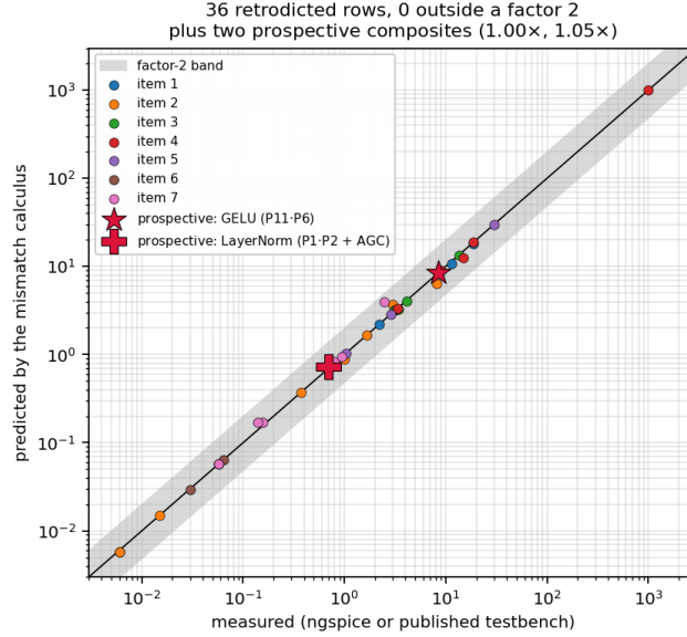
Figure 1: Pre-registered test of the mismatch calculus. Grey band: factor 2. Circles: the 36 retrodicted rows, grouped by item; none falls outside the band, worst 1.63\times . Red markers: the two prospective composites, predicted before the arbitrating circuit simulations were run ( 1.00\times and 1.05\times on the per-channel median). Figure regenerated from the stored numerical results; see spice/make_v3_figures.py .
