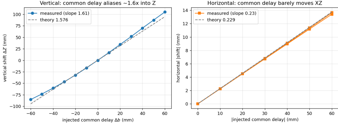
Figure 6: Empirical confirmation of the common-delay-to-vertical alias. Injecting a known common-mode range offset \Delta b into the static ranges and re-localizing without modelling it shifts the recovered position: the vertical shift tracks \Delta b at slope 1.61 (closed-form geometric prediction 1.58), while the horizontal shift grows at only 0.23 per unit |\Delta b| , the UWB analogue of the GPS receiver-clock/altitude coupling. Source: literature_search/delay_injection_sweep.png .
