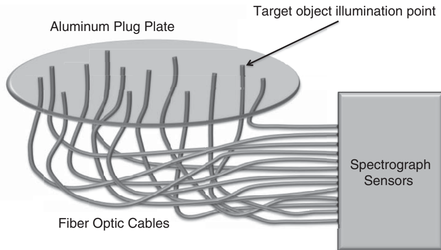
Figure 18.1: Aparatus for spectrographic analysis of stellar objects using an aluminum plug plate and fiber-optic cables. The aluminum plug plate is placed in the focal plane of a telescope.
