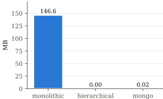
Python heap after reopening, N = 200
