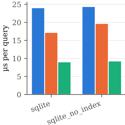
find_by_id
