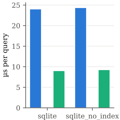
find_by_id, N = 100k
