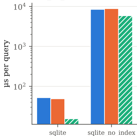
find_by_author (log scale)
