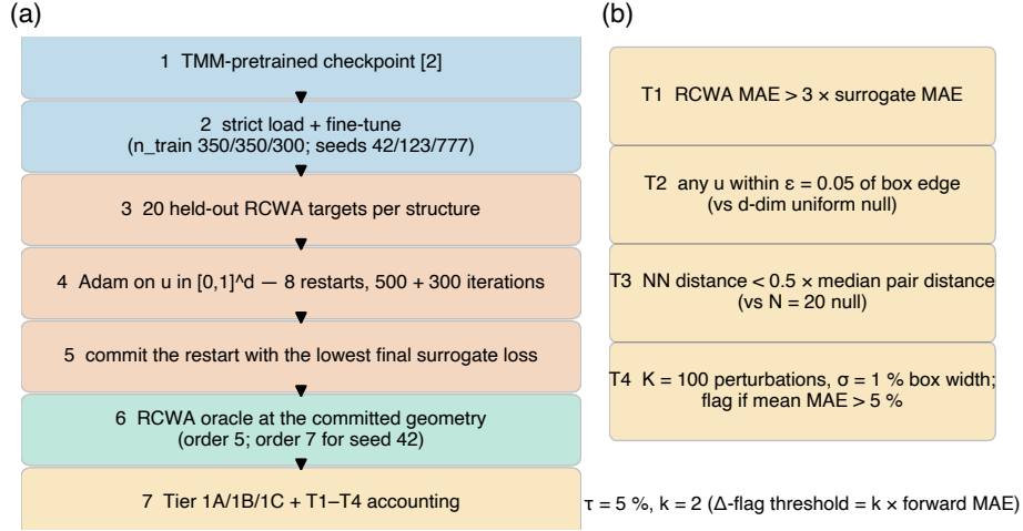
Figure 1: Protocol overview. (a) Pipeline: the TMM-pretrained checkpoint regenerated with the recipe of [1] is strict-loaded and fine-tuned (n_train 350 per structure; training seeds 42/123/777); 20 held-out RCWA targets per structure are inverted by Adam on the normalized geometry u with 8 restarts (500 + 300 iterations); the restart with the lowest final surrogate loss is committed; the committed geometry is evaluated once by the RCWA reference solver at its per-wavelength adaptive order; Tier 1A/1B/1C and the T1–T4 taxonomy are accounted. (b) Pre-specified thresholds: \tau = 5\% , k = 2 ( \Delta -flag threshold = k \times forward MAE), T1 factor 3, T2 \varepsilon = 0.05 , T3 factor 0.5, T4 K = 100 perturbations with \sigma = 1\% of the box width and a 5 % mean-MAE flag.
