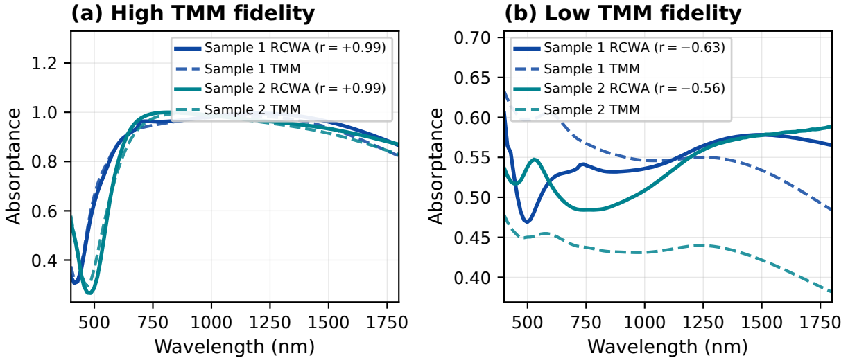
Figure 2: Representative TMM (dashed) vs. RCWA (solid) absorbance spectra for Structure A; each panel shows two parameter sets, with each sample drawn in a distinct hue and the RCWA/TMM pair sharing that hue (legend lists the per-sample Pearson correlation r ). (a) High-fidelity cases ( r \approx 1.0 ) where TMM closely tracks the RCWA cavity resonance. (b) Low-fidelity cases ( r \approx -0.6 ) where RCWA exhibits sharp resonance features that the planar TMM cannot reproduce.
