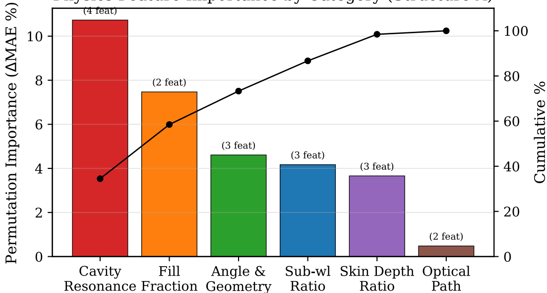
Physics Feature Importance by Category (Structure A)
