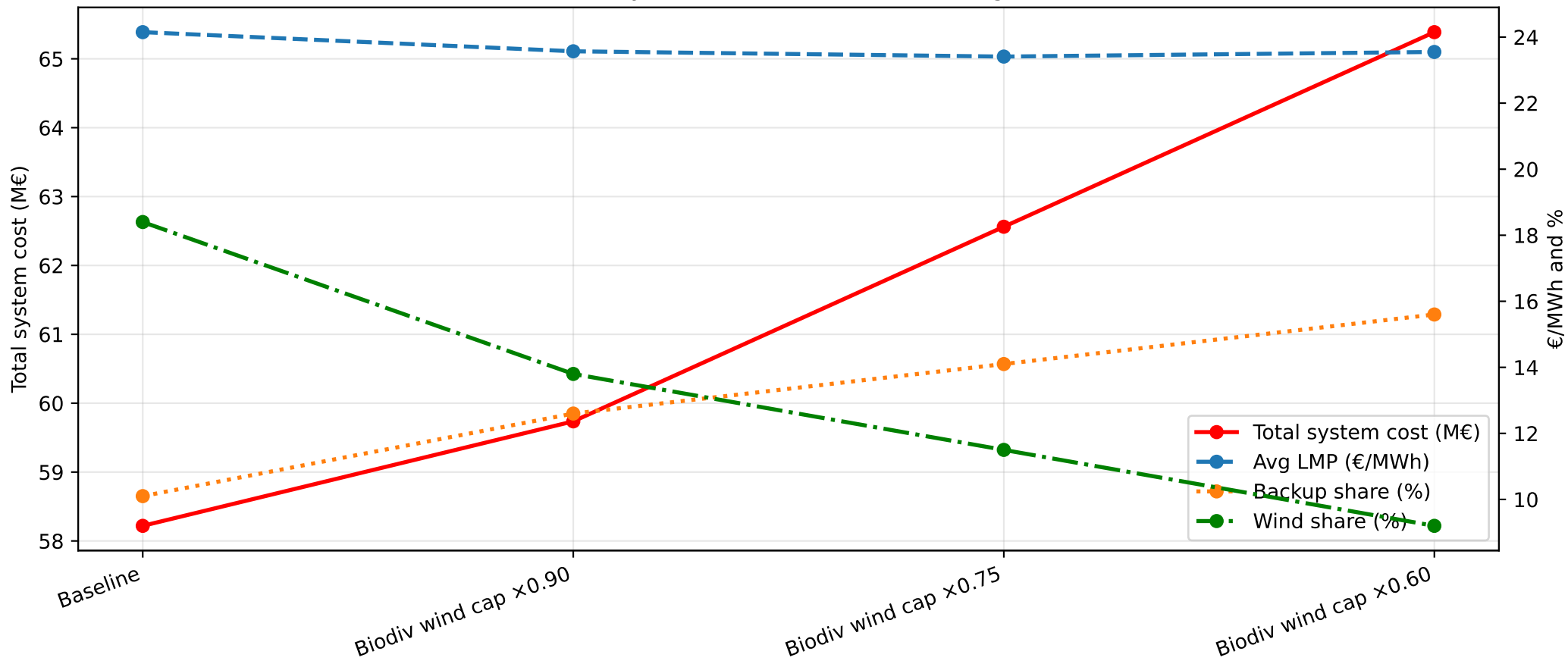
Baseline vs Biodiversity-aware wind constraints (Belgium, March 2013)
