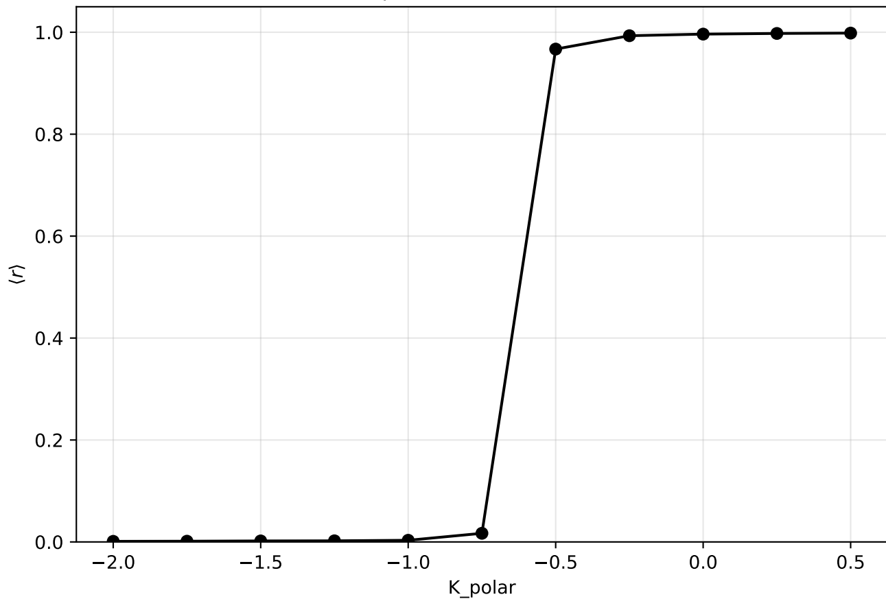
Order parameter vs frustration
