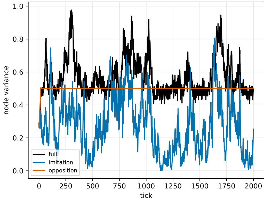
Cross-node variance
