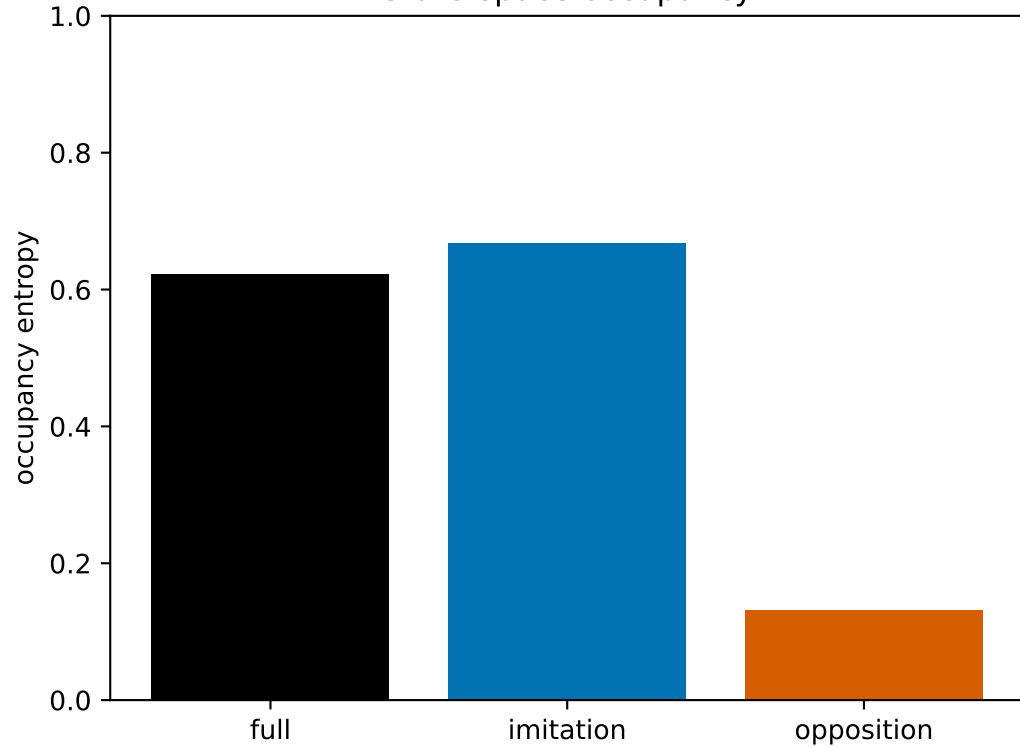
State-space occupancy
