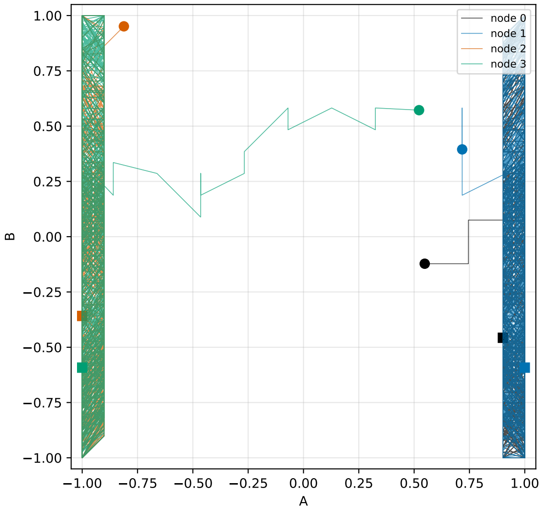
SCM phase portrait
