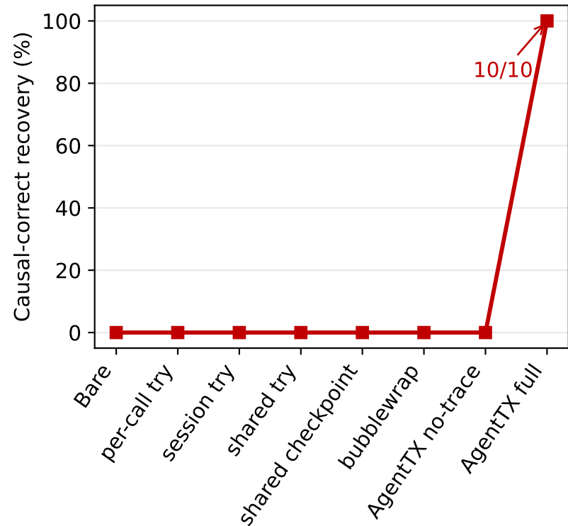
10 fresh-workspace repeats
