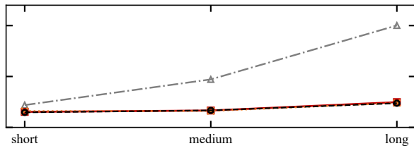
SWE tasks by clean-solve cost (a) Session only
