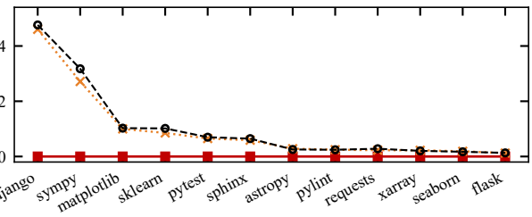
Repository, ordered by task count (d) Replay, summed
