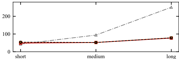
SWE tasks by clean-solve cost (a) Session + replay, summed
