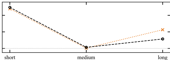
SWE tasks by clean-solve cost (c) Summed extra after replay
