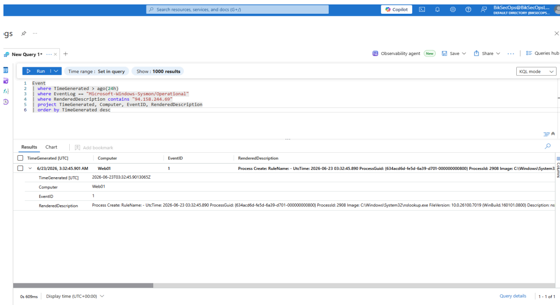
Fig 12 -- Sentinel Logs: IOC Hunt results -- 1 result for 94.158.244.69 -- nslookup.exe (C:\Windows\System32\nslookup.exe) captured, RenderedDescription showing full process details
