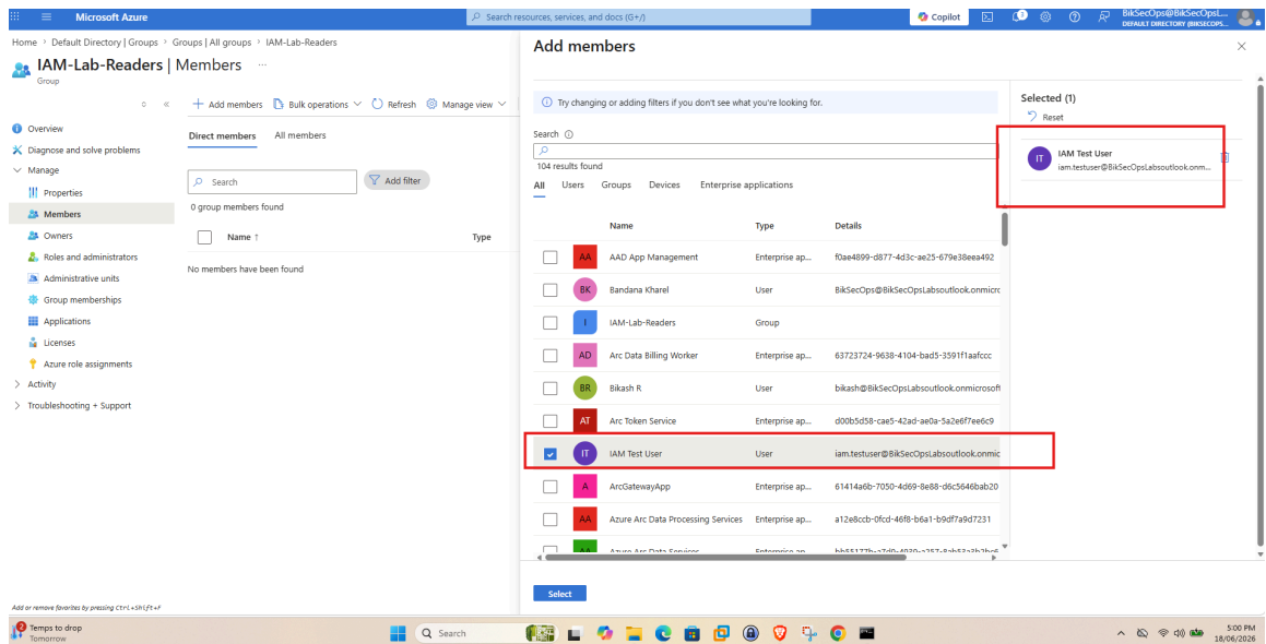
Fig 6 -- Entra ID: Add members -- IAM Test User selected to join IAM-Lab-Readers
