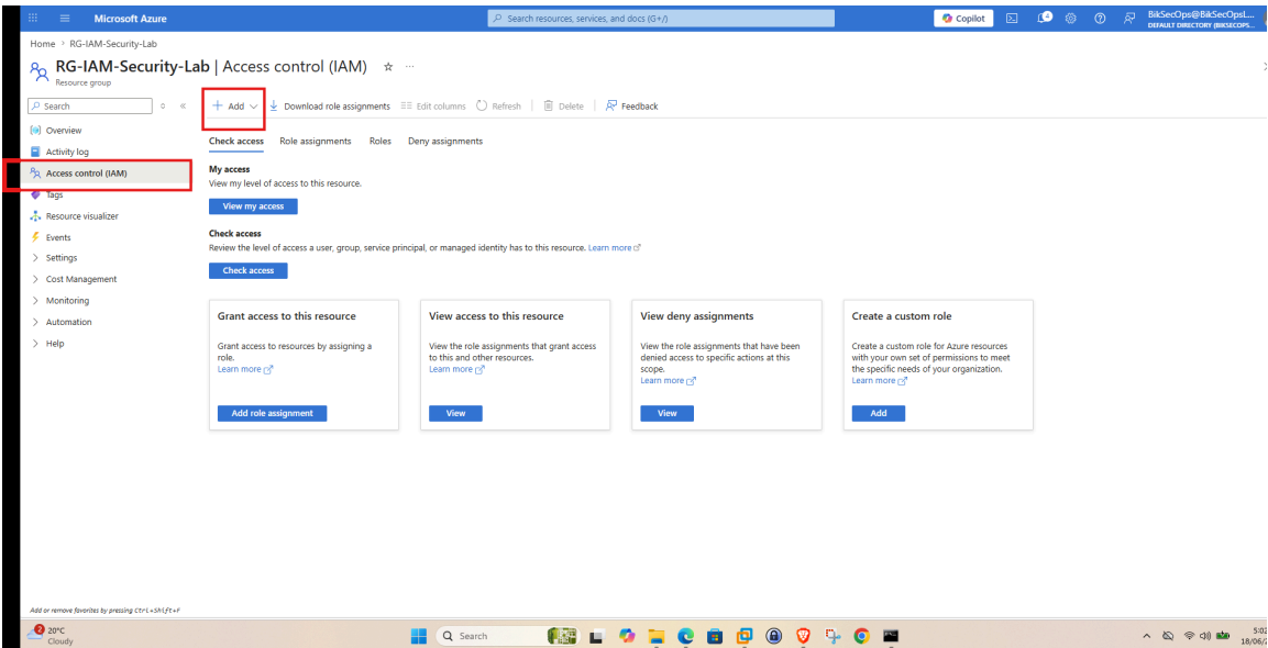
Fig 8 -- Azure Portal: RG-IAM-Security-Lab Access Control (IAM) -- Add role assignment highlighted
