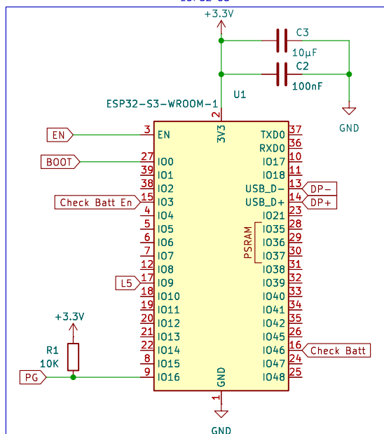
ESP32 S3
