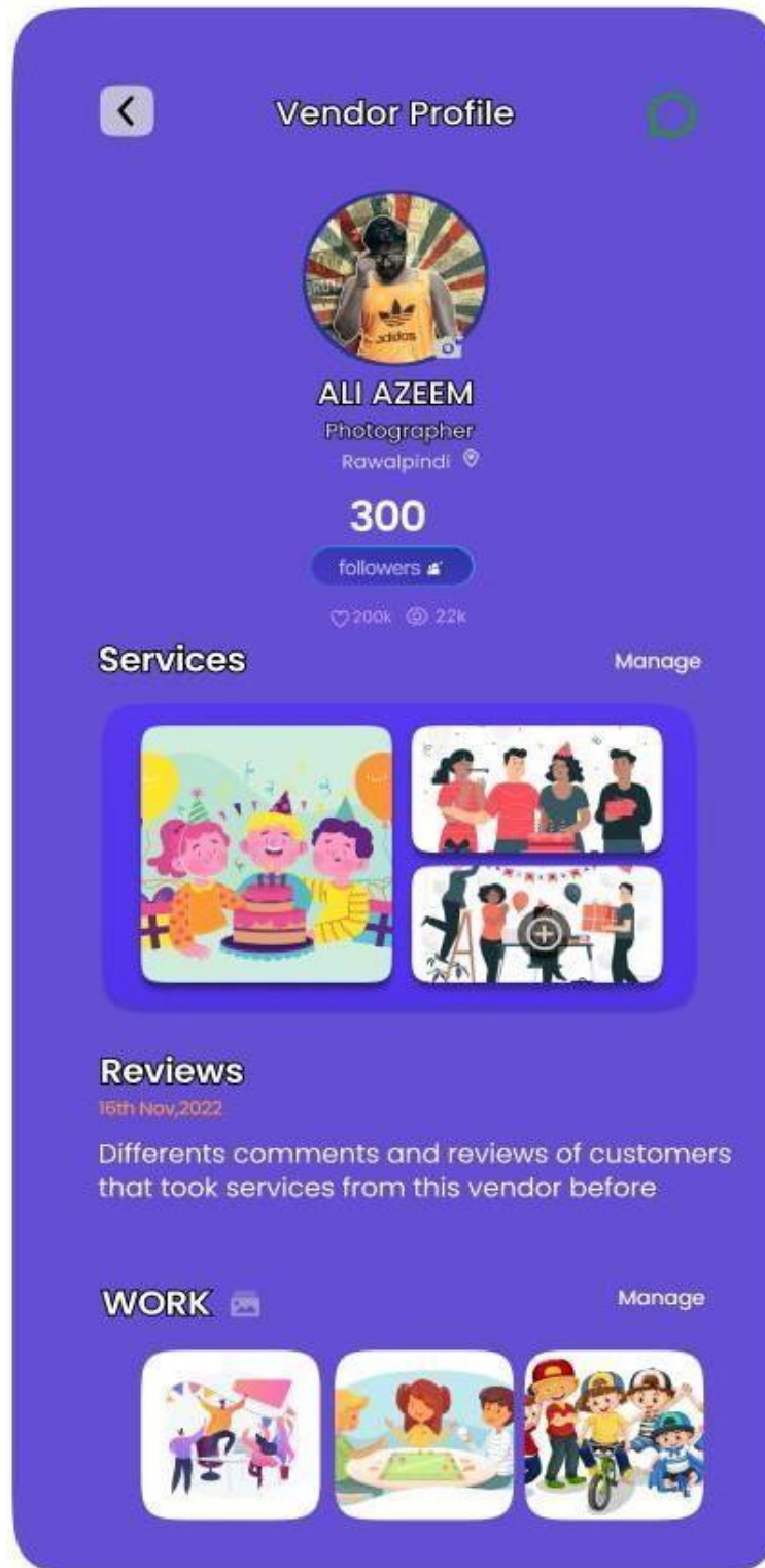
Figure 2-23 Vendor Profile
