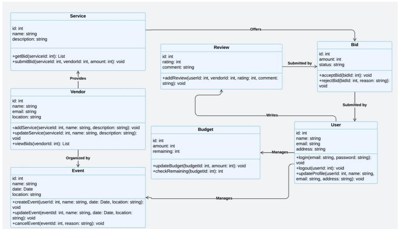
Figure 3-2 Class Diagram
