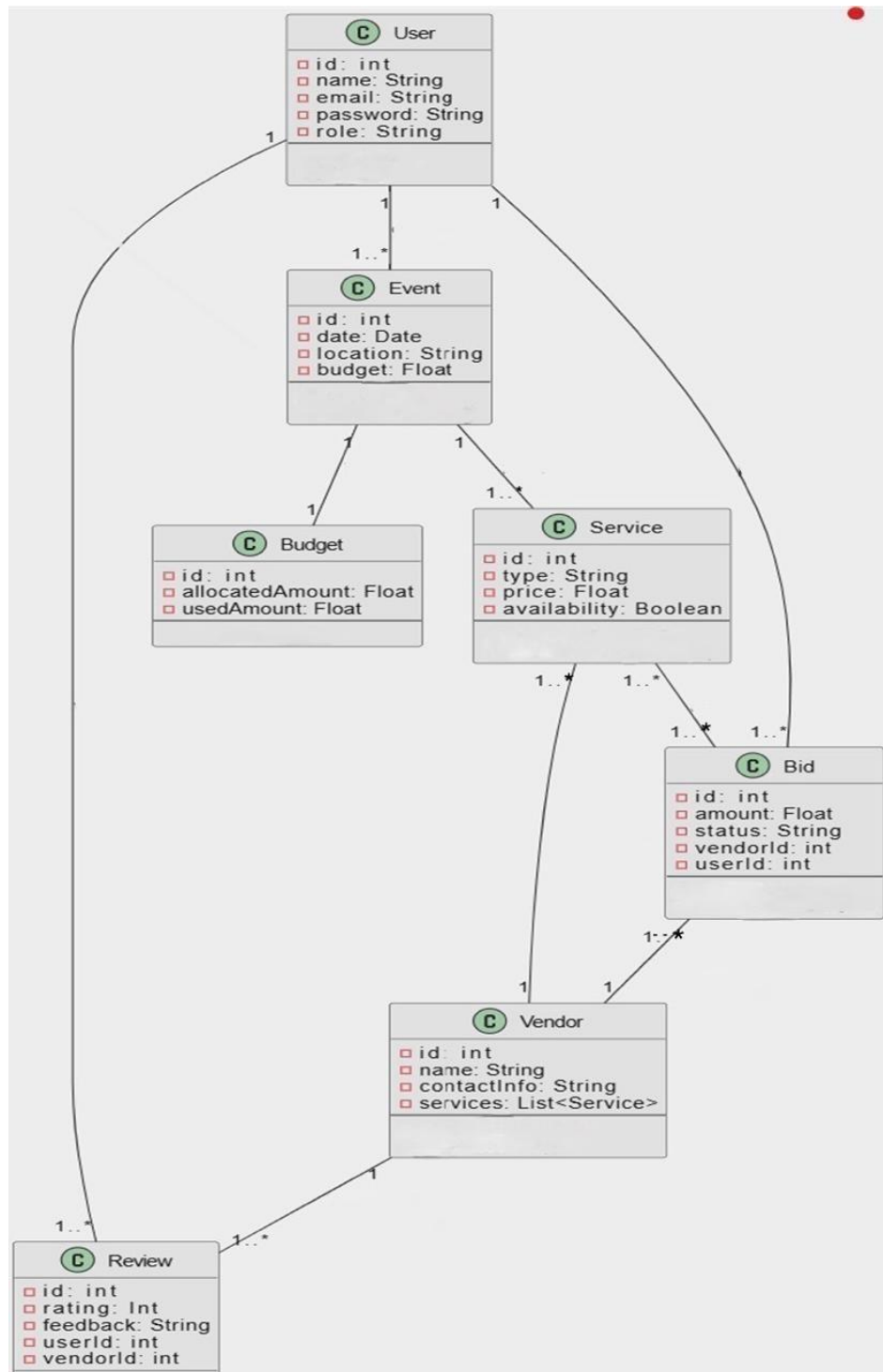
Figure 2-15 Domain Model
