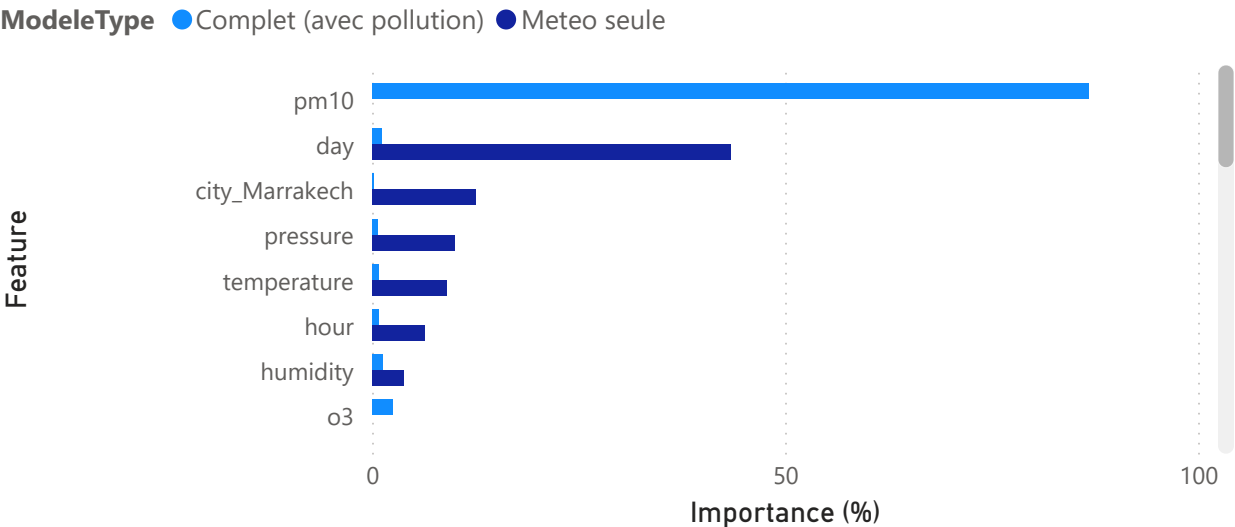
Importance des features (Top 10)
