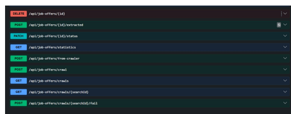
FIGURE 4.27 – Documentation Swagger — Job Offer Service (suite)
