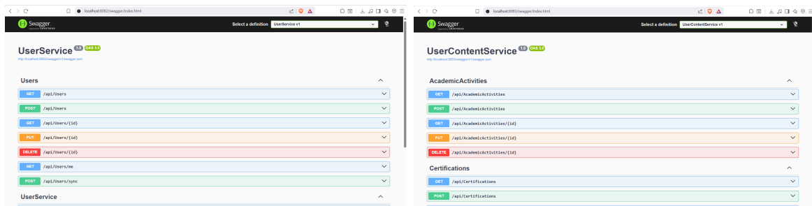
FIGURE 4.23 – Documentation Swagger — User Service et User Content Service
