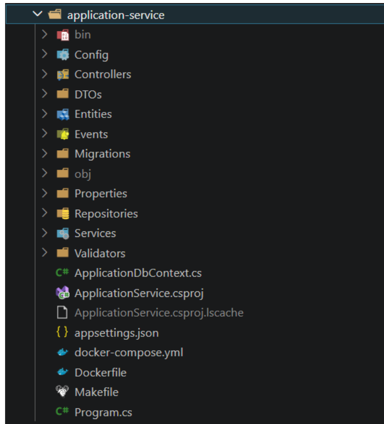
FIGURE 4.15 – Structure du Application Service
