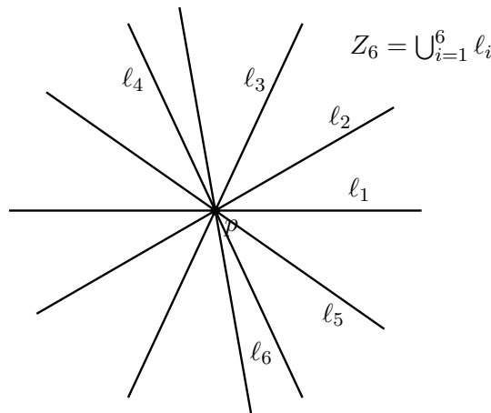
Figure 2.1: An example of a 6-cross in \mathbb{P}^3 .
