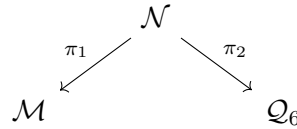
Figure 4.4: Incidence diagram for the projections \pi_1 : \mathcal{N} \rightarrow \mathcal{M} and \pi_2 : \mathcal{N} \rightarrow \mathcal{Q}_6 .
