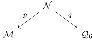
Figure 4.4: Incidence diagram with the morphisms p : \mathcal{N} \rightarrow \mathcal{M} and q : \mathcal{N} \rightarrow \mathcal{Q}_6 .
