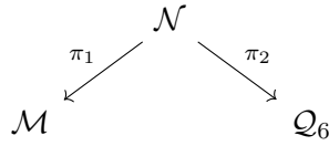
Figure 3.4: Incidence diagram for the projections \pi_1 : \mathcal{N} \rightarrow \mathcal{M} and \pi_2 : \mathcal{N} \rightarrow \mathcal{Q}_6 .
