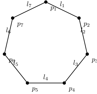
Figure 2.2: Schematic k -gon (here k = 7 ) drawn in a plane; each vertex is an intersection point p_i and the line segments represent the lines l_i .
