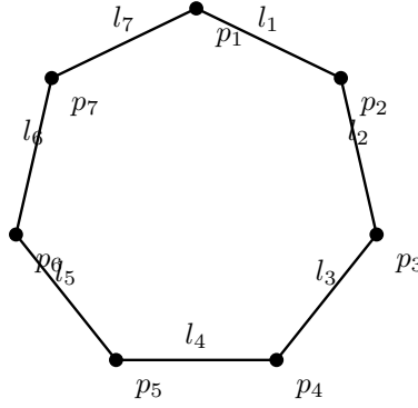
Figure 3.2: 7-gon drawn in a plane; each vertex is an intersection point p_i and the line segments represent the lines l_i .
