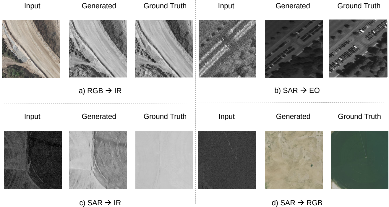
Figure 1. Qualitative results on our hold-out validation set from the official train set. (a) RGB \rightarrow IR, (b) SAR \rightarrow EO, (c) SAR \rightarrow IR, (d) SAR \rightarrow RGB. Each panel shows input, generated output, and ground-truth target. EarthBridge preserves structural integrity while synthesizing high-fidelity textures across Electro-Optical (EO), Infrared (IR), and Synthetic Aperture Radar (SAR) modalities.
