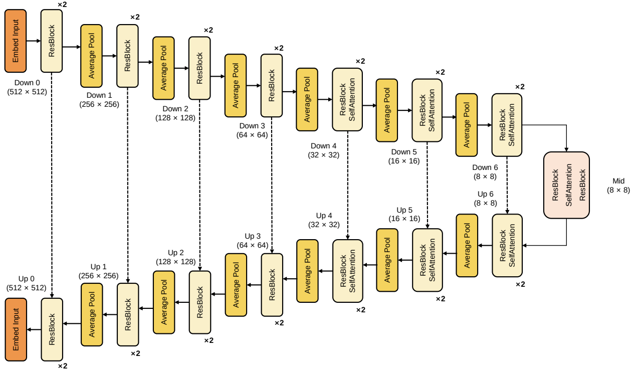
Figure 4. UNet denoiser architecture for 1024px tasks (SAR→RGB, RGB→IR). The encoder downsamples via ResBlocks and average pooling; the decoder upsamples with skip connections. Source \mathbf{x} is channel-concatenated with \mathbf{z}_t ; the output is \hat{\mathbf{z}}_0 . We train at 512 \times 512 and infer at full resolution.
