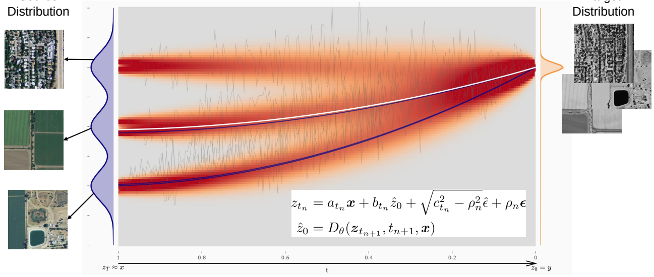
Figure 2. Distribution evolution of the diffusion bridge. The source distribution at z_T = \mathbf{x} (left) converges through time t to the target distribution at z_0 = \mathbf{y} (right), governed by the DBIM update rule and denoiser D_\theta .
