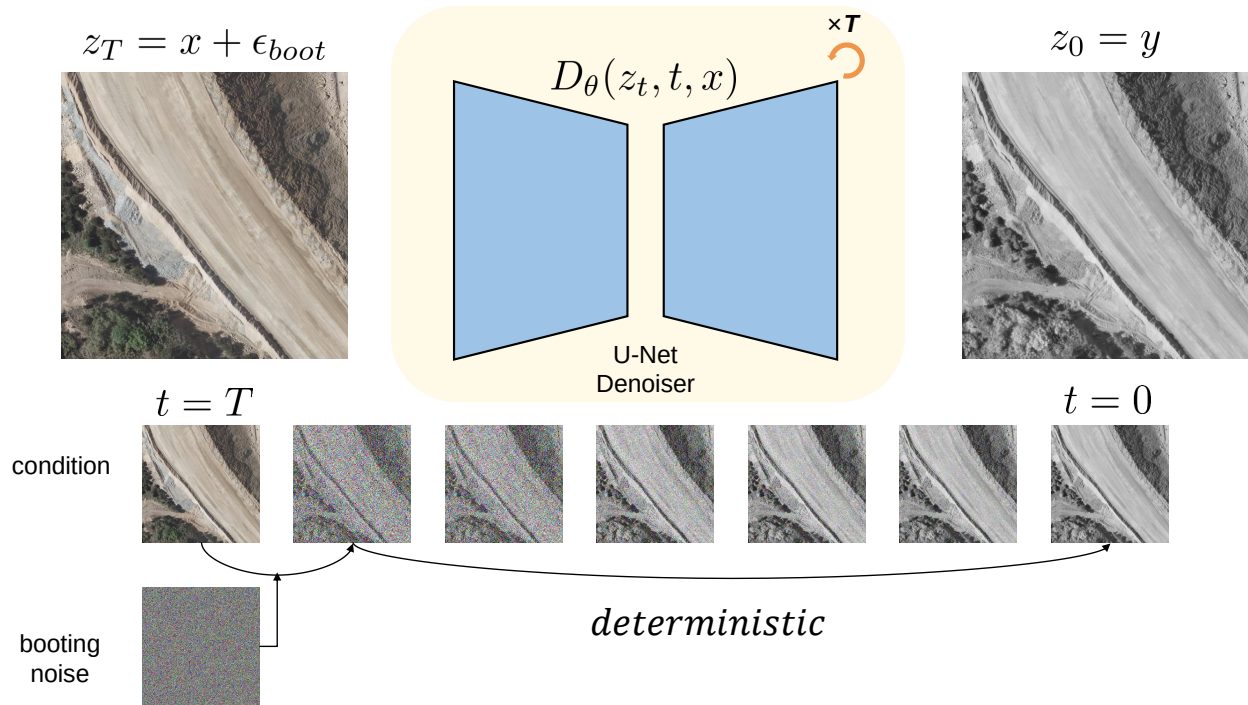
Figure 3. Deterministic DBIM sampling. The noisy input z_T = \mathbf{x} + \epsilon_{boot} is progressively denoised by D_\theta(z_t, t, \mathbf{x}) to produce the clean output z_0 = \mathbf{y} . The step sequence shows conditioning, booting noise injection, and gradual refinement from t = T to t = 0 .
