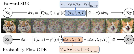
Figure 1: A schematic for Denoising Diffusion Bridge Models. DBM uses a diffusion process guided by a drift adjustment (in blue) towards an endpoint x_T = y . They learn to reverse such a bridge process by matching the denoising bridge score (in orange), which allows one to reverse from x_T to x_0 for any x_T = y \sim q_{\text{data}}(y) . The forward SDE process shown on the top is unidirectional while the probability flow ODE shown at the bottom is deterministic and bidirectional. White nodes are stochastic while grey nodes are deterministic.
