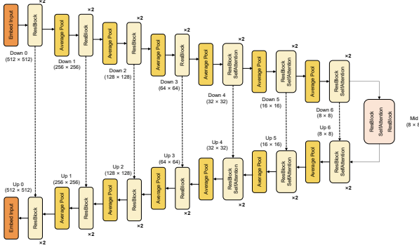
Figure 1. UNet architecture of our DBIM for 1024px tasks (SAR→RGB, RGB→IR). We train at 512 \times 512 and infer at full resolution. Source x is channel-concatenated with noisy sample z_t and processed by this denoiser. Bridge scalings a_t, b_t, c_t construct z_t during training; deterministic DBIM sampling generates \hat{z}_0 during inference.
