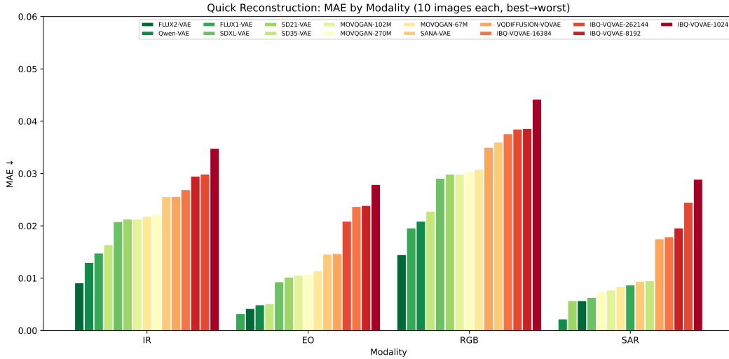
Figure 2: Quick reconstruction: MAE by modality (10 images each). VAEs ordered best→worst; color indicates performance (green=best, red=worst).
