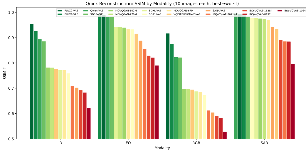
Figure 3: Quick reconstruction: SSIM by modality (10 images each). VAEs ordered best→worst; color indicates performance (green=best, red=worst).
