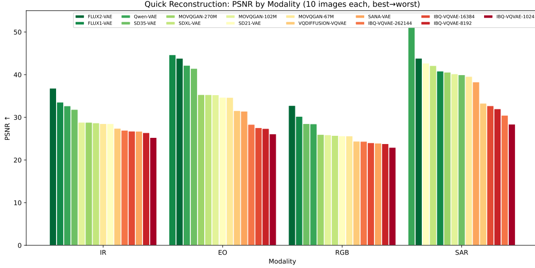
Figure 1: Quick reconstruction: PSNR by modality (10 images each). VAEs ordered best→worst by average rank; color indicates performance (green=best, red=worst).
