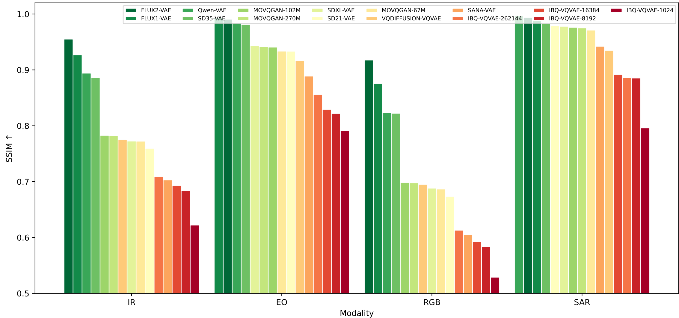
Quick Reconstruction: SSIM by Modality (10 images each, best→worst)
