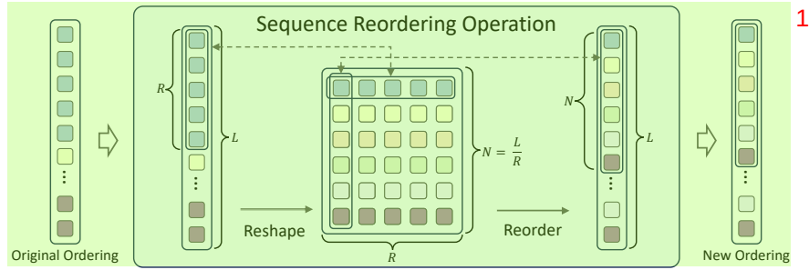
Fig. 2: Illustration of Sequence Reordering Operation. 2
