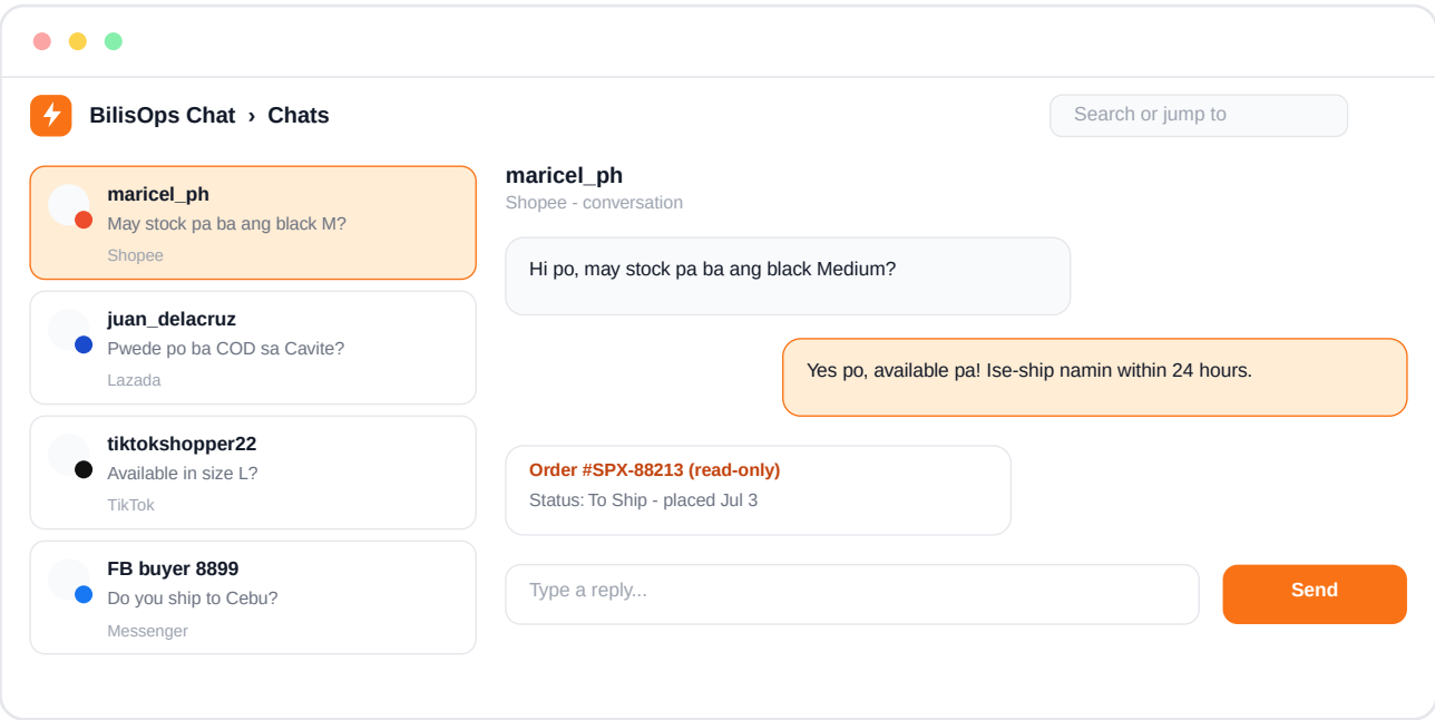
Illustration of the unified inbox: conversations from Shopee, Lazada, TikTok Shop and Messenger in one queue.
