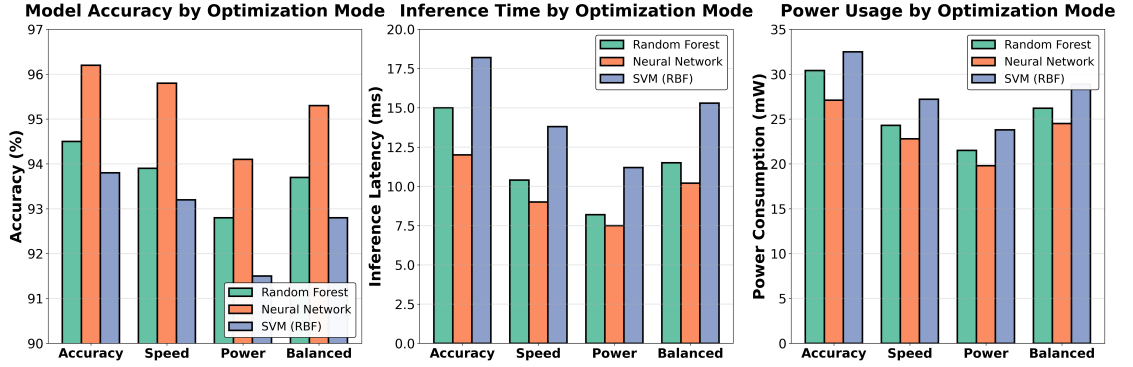
Figure 4.4.1: Comparative analysis of accuracy, inference latency, and power consumption across four optimization modes
