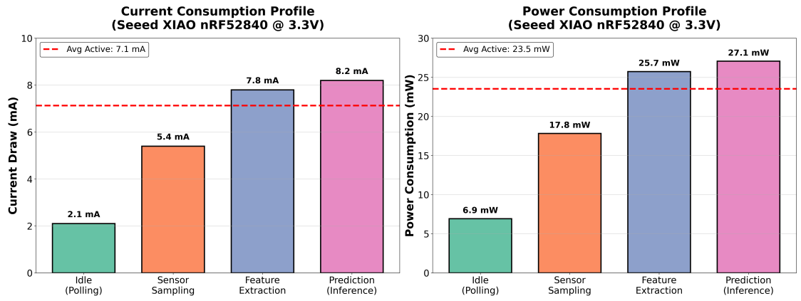
Figure 4.4.2: Power Consumption Profile During Inference (Neural Network, Accuracy Mode)
