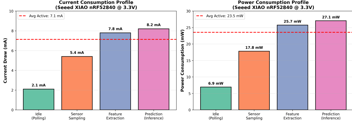
Figure 5: Power Consumption Profile During Inference (Neural Network, Accuracy Mode)
