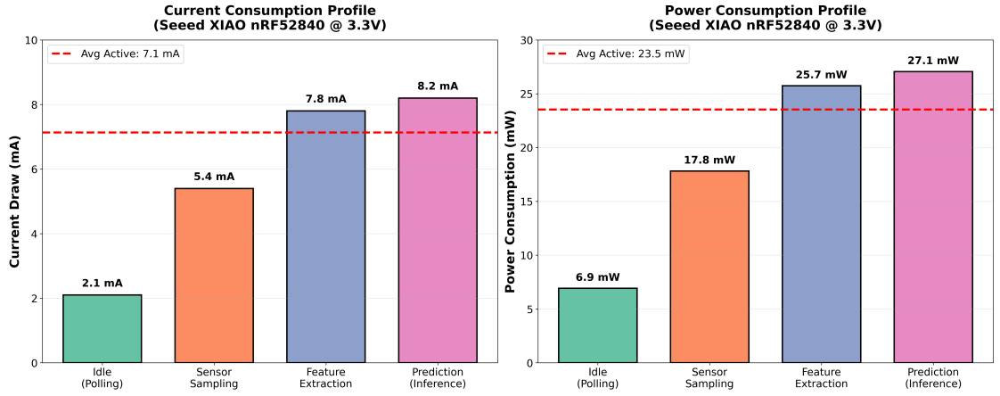
Figure 4.4.2: Power Consumption Profile During Inference (Neural Network, Accuracy Mode)
