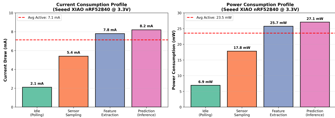
Figure 3: Power Consumption Profile During Inference (Neural Network, Accuracy Mode)
